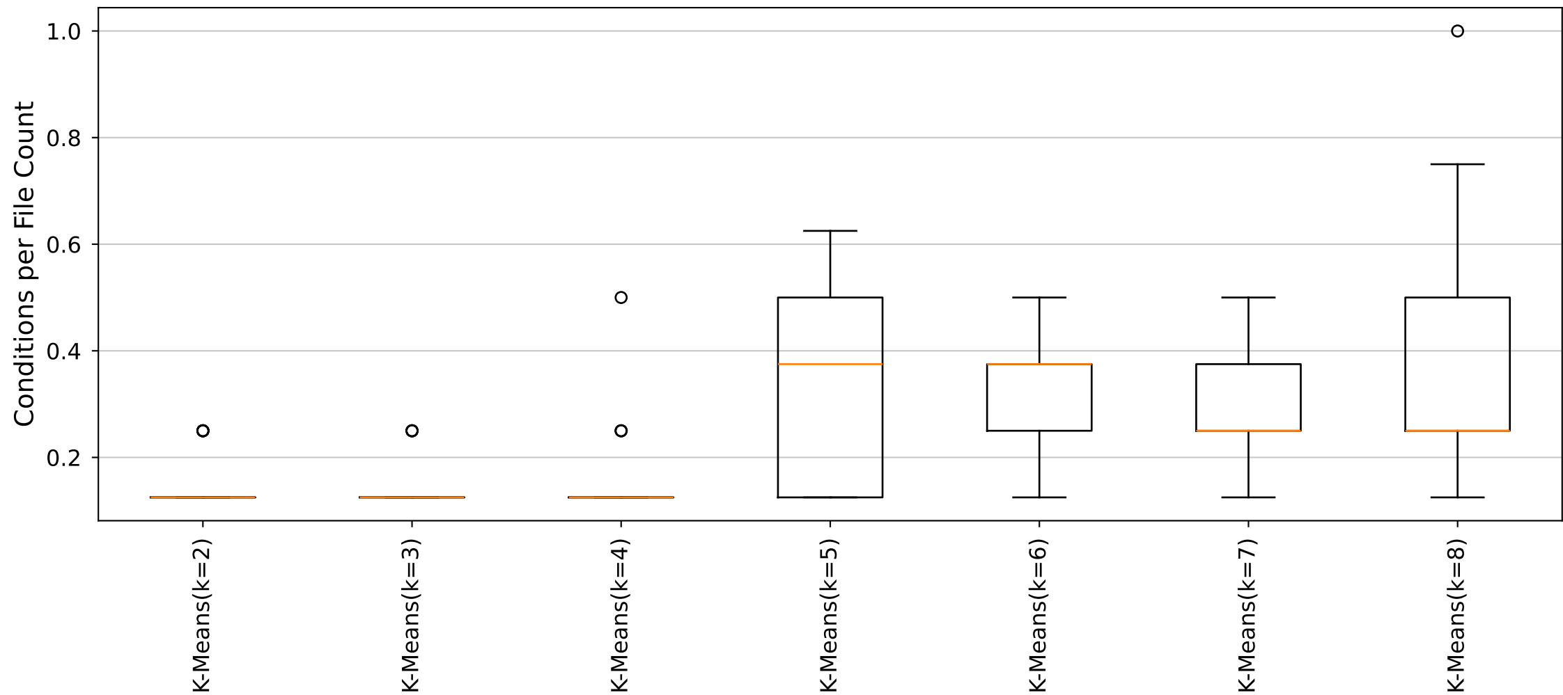
YARA Rules Conditions per File Count Distribution (Cluster16_Size8 dataset)
